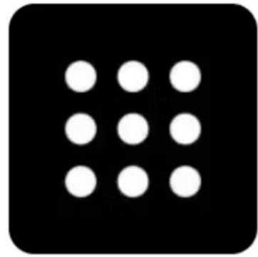
Perplexity
